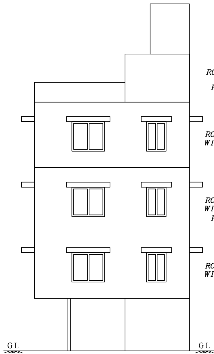
FRONT ELEVATION
