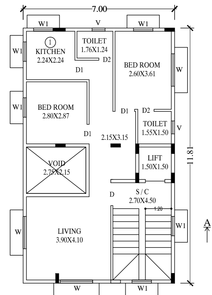
PROPOSED TYPICAL GROUND, FIRST & SECOND FLOOR PLAN
