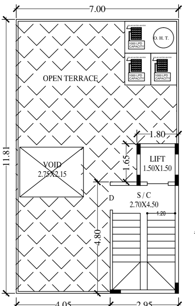
PROPOSED TERRACE FLOOR PLAN
